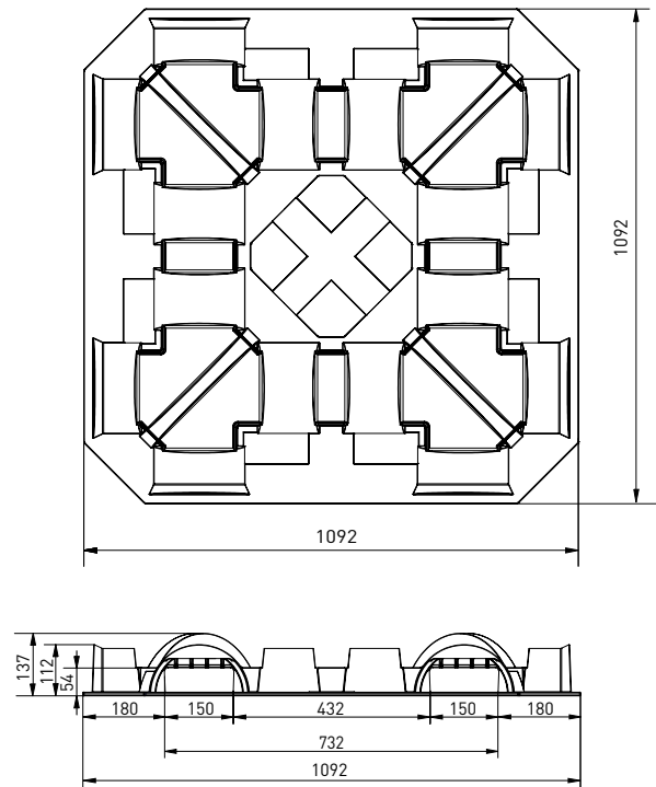
BigBag Divider 4343
