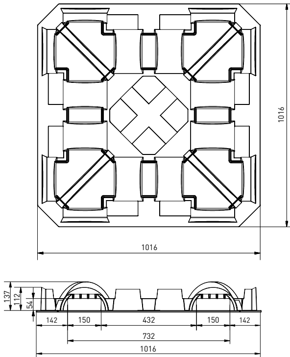
BigBag Divider 4040
